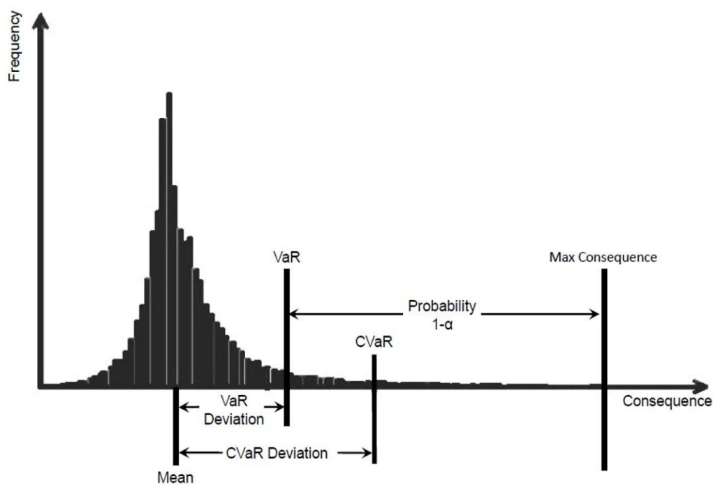
Figure 1: VaR and CVaR Deviations [Source: Sarykalin et al (2008)]
